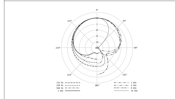
Frequency response curve M149
